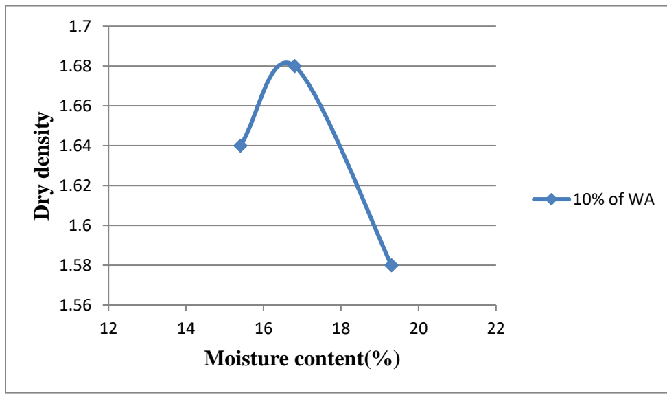
Fig 4.13 Dry density vs moisture content of 10% of Wooden ash and soil
