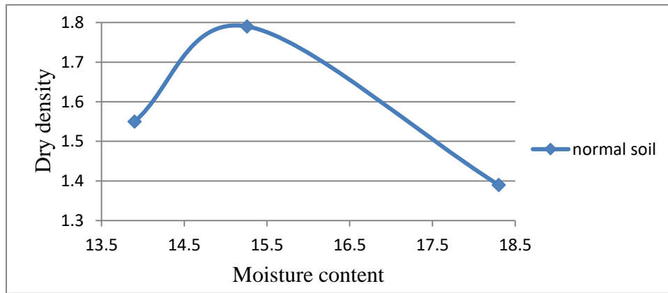
Fig 4.1 Dry density vs moisture content for the normal soil
