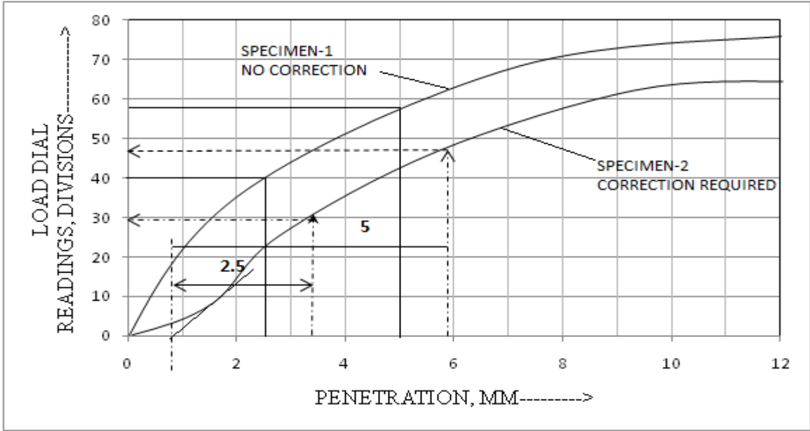
Load-penetration curve for CBR test
